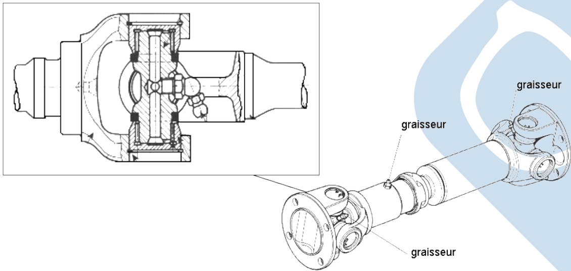
Joint de cardan GLAENZER SPICER
